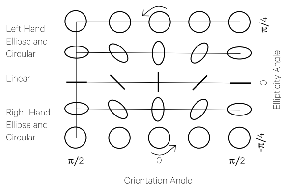
Figure 8.24 Various polarisations of transmitted and received signals
